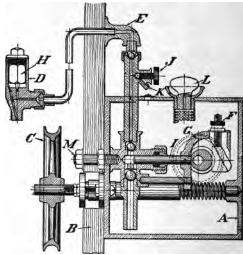
FIG. 394.—Section Through a Type of Power Driven Oil Pump. A, oil reservoir; B, dashboard of car; C, pulley driven by belt from engine shaft; D, gravity valve on distributor; E, outlet elbow; F, set screw to regulate stroke of plunger, I; G, plunger bracket bearing against eccentric, which is on the gear operated by worm, or endless screw, on the shaft of pulley; C; H, weight of gravity valve, D, for holding outlet port normally closed, and rising under pressure of oil from pump; I, plunger of pump drawing oil from reservoir, A, through ball valve, and expelling it through ball valve to outlet, E; J, test cap for testing flow of oil; K, oil outlet for test cap; L, filling plug and strainer; M, stud bolt for securing machine to dashboard.
